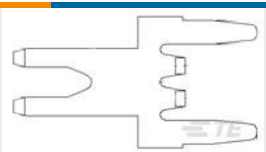
TE 产品编号1217041-1 TAB, POKE IN PCB 020 TPCUBR
