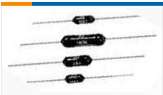
TE 产品编号1879628-8 H4P 270K 1% 100PPM
