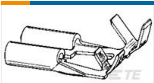
TE 产品编号170191-3 FF 312 REC 18-14AWG TPBR REREELING
