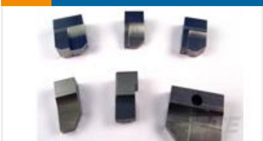
TE 产品编号3-1333207-1 ANVIL, COMBINATION .110
