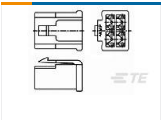
TE 产品编号174202-1 250 FASTON HSG., REC., 4 POS, NATURAL
