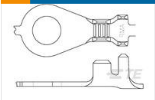
TE 产品编号444151-2 RING TONGUE 2.5-4.0 MM2 0.81 ELECTROTPBR
