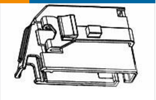
TE 产品编号284142-1 6 POS. FRAME INLINE 3.5 MM PIT
