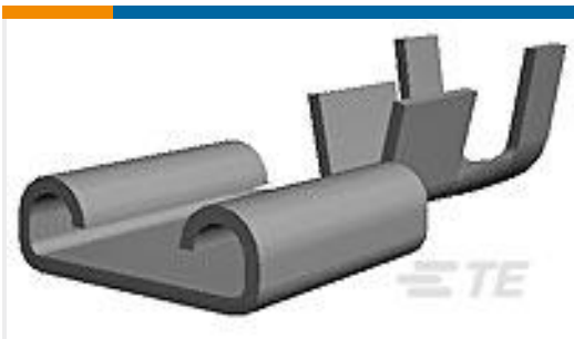
TE 产品编号170179-2 205 FASTON, REC., 18-14 AWG, TPBR
