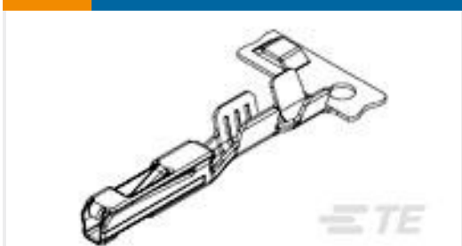
TE 产品编号1326028-2 0.64MM FEMALE CONTACT,AU, 22AWG
