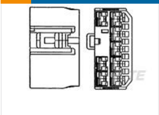
TE 产品编号175979-1 FF 187 PLUG HSG 8P NYLON NAT
