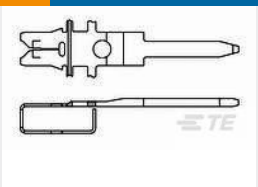
TE 产品编号1742633-1 TAB,.063 X .032,300 SERIES,MAG
