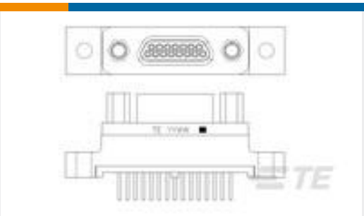
TE 产品编号1532267-2 M83513/22-B01CP = MCKS-C2-P-15PST1
