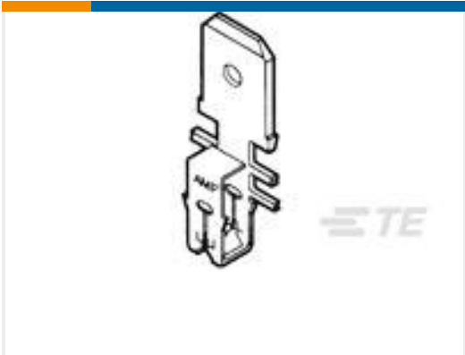
TE 产品编号62657-1 MAG-MATE 250FTAB 27-23 016TPBR
