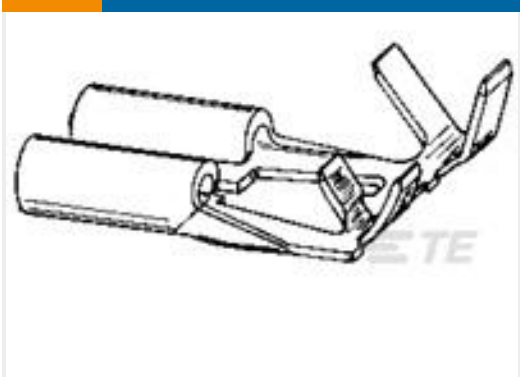
TE 产品编号180398-2 FF 250 REC 1-2.5MM2 TPBR
