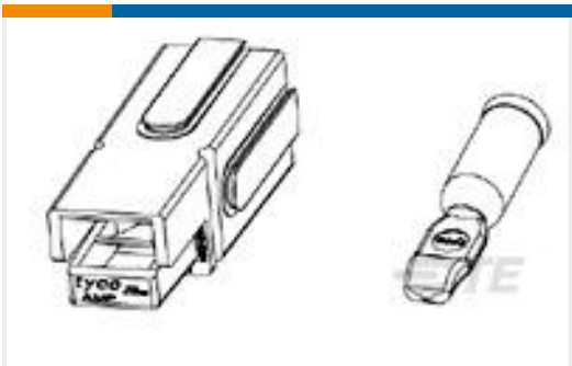
TE 产品编号1604002-2 120A SGL POLE KIT, 2 AWG BLACK
