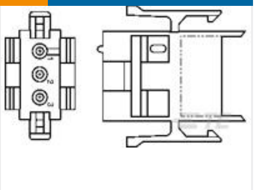
TE 产品编号1-640508-0 03P MR II CAP HSG V0 RED
