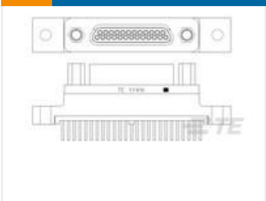
TE 产品编号1532269-1 M83513/22-D01CN = MCK5-C2-B-25PST1
