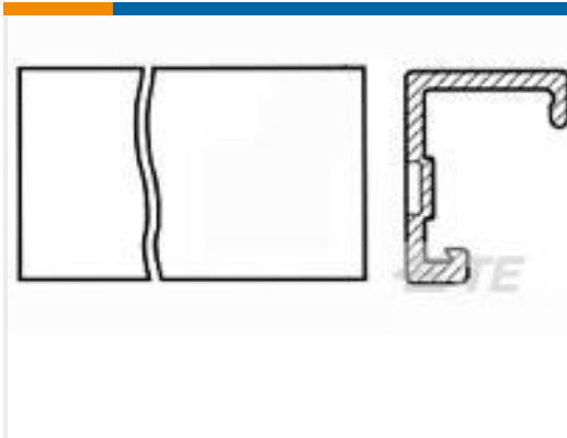
TE 产品编号1-640551-3 13P MTA156 COVER
