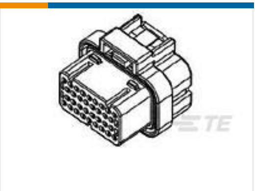
TE 产品编号1473712-2 SUPER SEAL 2ROW 26POS PLUG ASS
