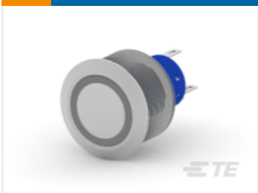
TE 产品编号1-2317656-1 AV25 SPL 3A MOVING RING WHITE 12V
