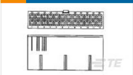
TE 产品编号1-1586862-8 18P FH PLUG VAL-U-LOK FH GW
