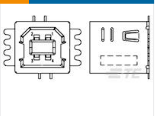
TE 产品编号1734517-1 STD USB TYPE B, VERTICAL, SMT, GRD FINGER
