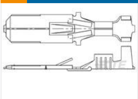
TE 产品编号160451-2 FF 250 TAB 18-14AWG TPPB LP
