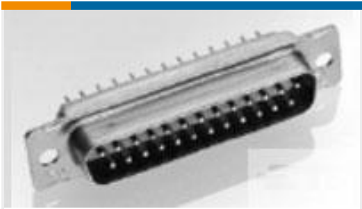
TE 产品编号1757829-2 AMPLIMITE,PLUG ASY,POSTD,109,ZN,2
