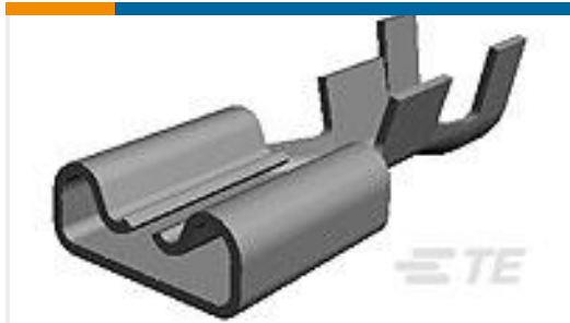
TE 产品编号1742198-1 250 FASTON,REC.,18-14 AWG,NPST
