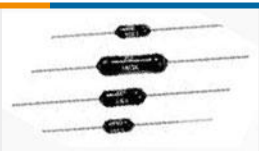
TE 产品编号1-1879629-1 H4P 220K 0.5% 50PPM
