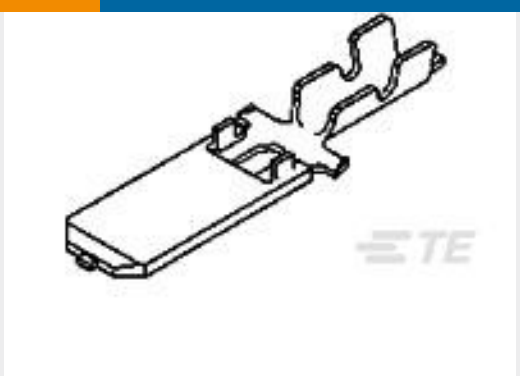
TE 产品编号170341-3 FF 250 TAB 14-12AWG PTBR WITHOUT LATCH
