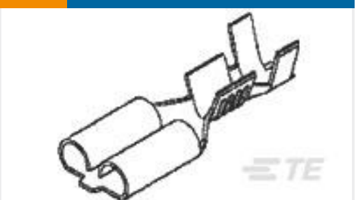
TE 产品编号170258-2 FF 250 REC 14-12AWG TPBR REREELING
