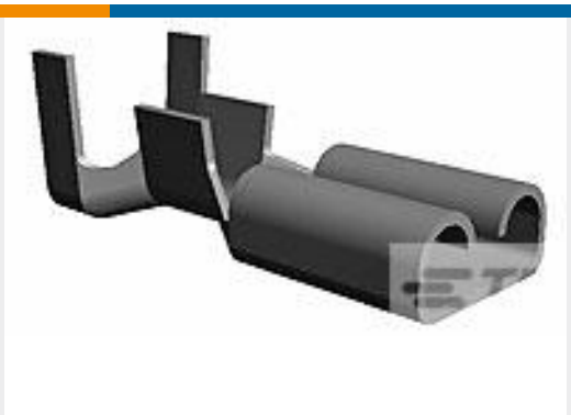
TE 产品编号170038-2 187 FASTON,REC.,20-16 AWG,TPBR
