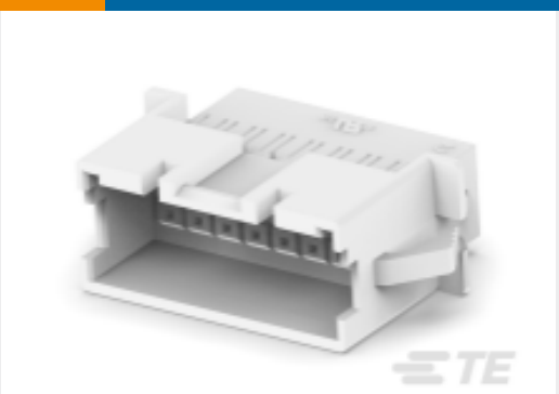
TE 产品编号1-2324584-6 HSG,REC,PANEL MOUNT,DUALROW, EP2.5
