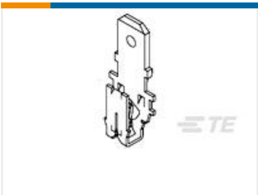
TE 产品编号1742035-1 TAB,187 X 032 FASTON,MAG-MATE
