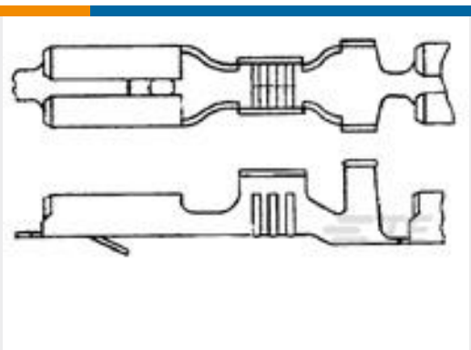
TE 产品编号170015-2 FF 110 REC 20-16AWG BR REREELING
