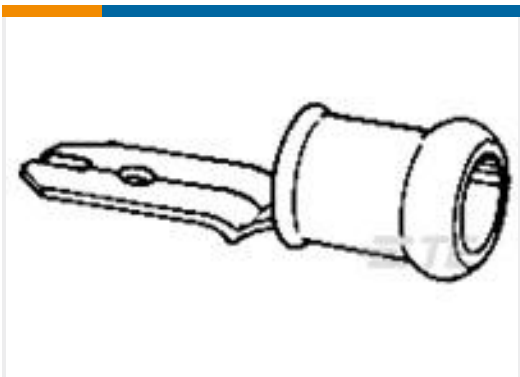
TE 产品编号140896-2 TERMINAL TAB FASTON PIDG 6,35
