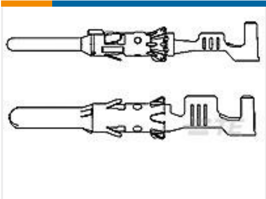
TE 产品编号1703018-1 DIA 1.5MM CONTACT PIN, LP
