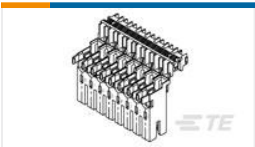
TE 产品编号1-770894-0 3.96mm Wire-to-board housing: receptacle, with mating alignment, SL 156
