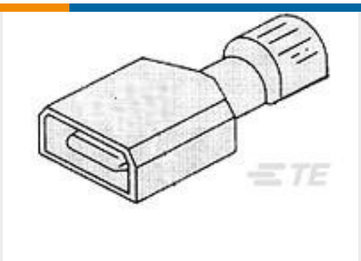
TE 产品编号2-520102-2 ULTRA-FAST 250 ASSEMBLY TAB 22-18 AWG BR
