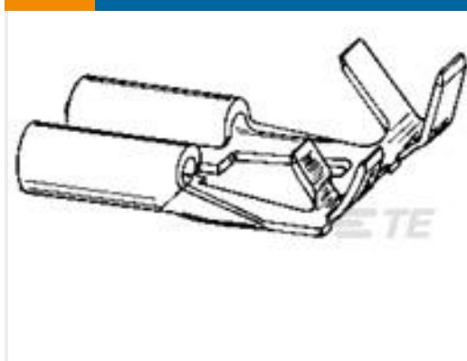
TE 产品编号170191-3 FF 312 REC 18-14AWG TPBR REREELING
