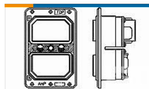
TE 产品编号1218476-1 MM2R106S106S-0100(201)ARINC404
