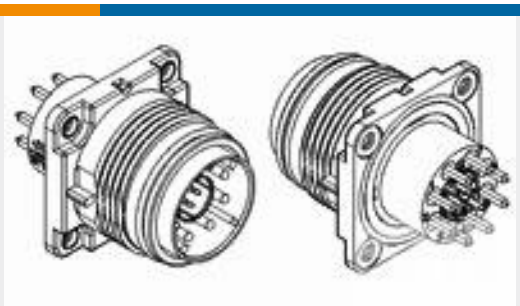
TE 产品编号1108846-1 HC26.Base Housing-PCB
