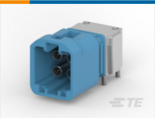
TE 产品编号2304168-3 4POS MATE-AX, HDR ASSY,90 DEG, COD C
