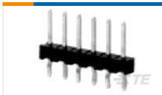
TE 产品编号104427-1 03 MODII HDR SRST B/A W/HLDWN PIN
