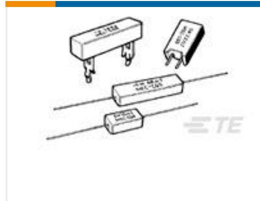
TE 产品编号1-1623788-3 SQM5 33R 5% (WIRE)
