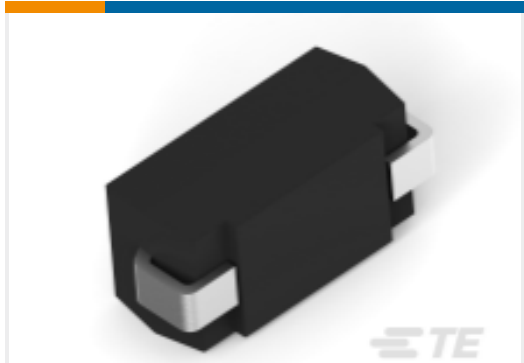
TE 产品编号2-2176323-4 SMV 2W 8M2 5%
