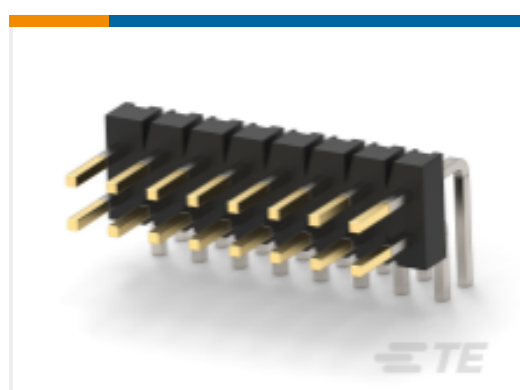
TE 产品编号5-146308-8 16 MODII HDR DRRR B/A .100
