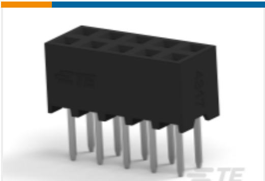
TE 产品编号1-2314820-0 10P,2MM,B-B,REC,DRV,T,2.7,0.1AU,TB
