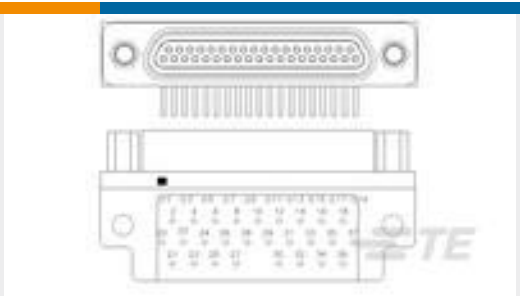
TE 产品编号1532263-3 M83513/13-F01NN = MCKS-N1-B-37SRT1
