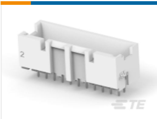
TE 产品编号2-2324245-2 ASSY,HDR,VERT,GWT,BOSSED,DUAL ROW, EP2.5
