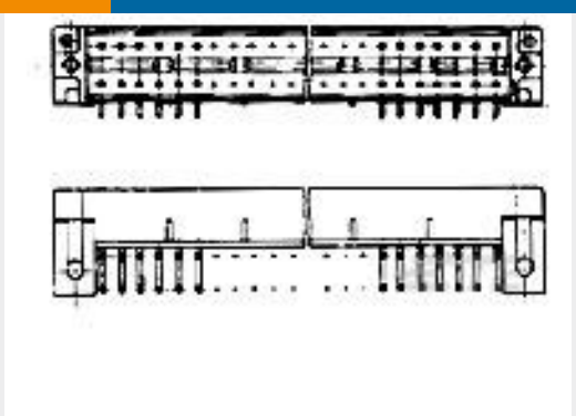
TE 产品编号172457-1 POST HDR ASSY 24P MULTI TAP
