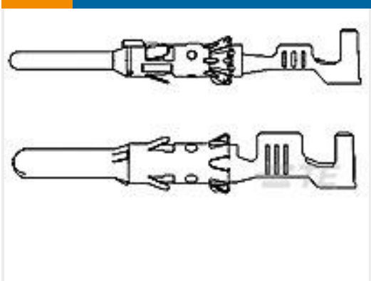
TE 产品编号1703013-8 DIA 1.5MM CONTACT PIN
