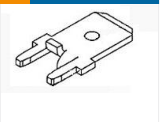
TE 产品编号1217167-1 250 FASTON,PCB TAB,TCBR
