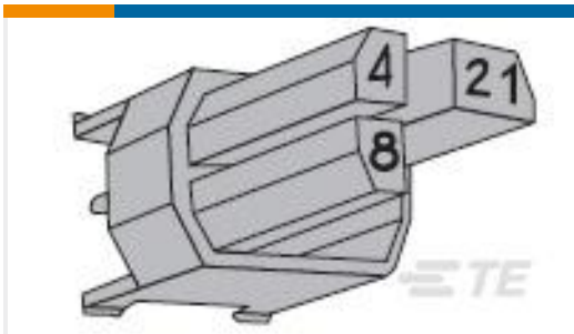
TE 产品编号172624-3 DRAWER CONN. MALE 24P 4.3MM
